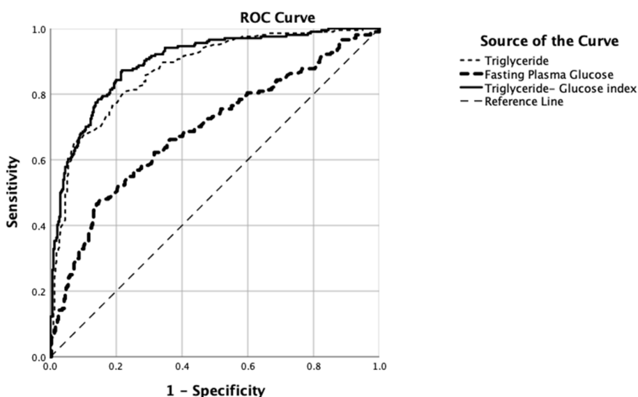
Fig. 7 The discriminatory power of the triglyceride-glucose index (TyG index) for metabolic syndrome by receiver operating characteristics (ROC) curve
